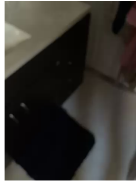
Laplacian 3
