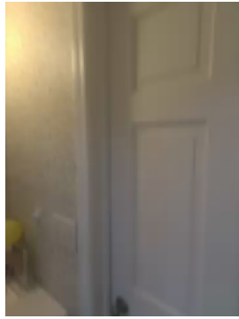
Laplacian 2
