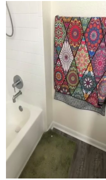
Laplacian 844
